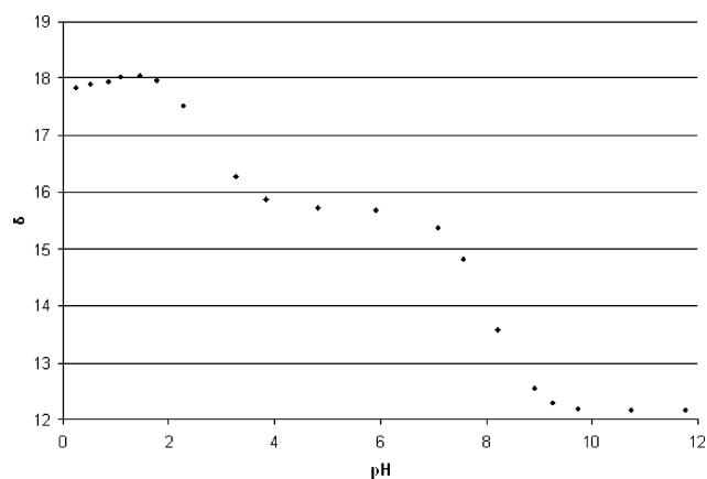
Figure 4. pH dependence of the chemical shifts \delta (ppm) of P- \beta of compound 6a .
