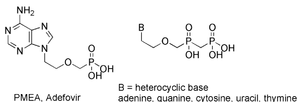
Figure 1. Acyclic analogues of nucleotides.
