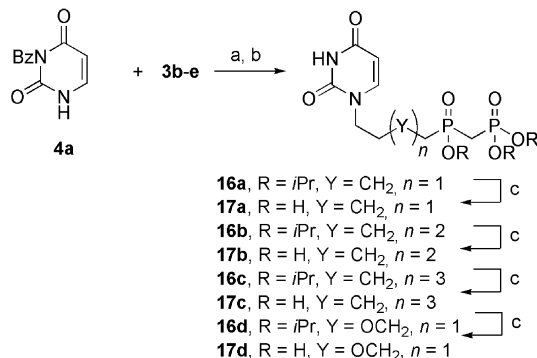
Scheme 3. Synthesis of analogues of dUDP. Reagents and conditions: a) Ph 3 P, DIAD, THF, b) MeONa, MeOH, c) BrSiMe 3 , CH 3 CN.
