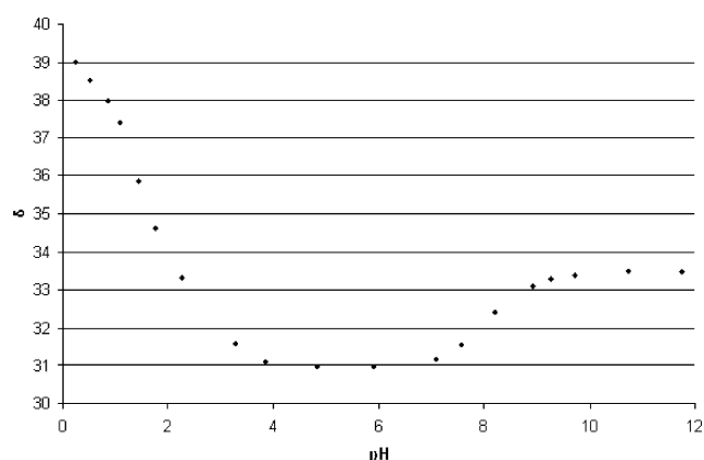
Figure 3. pH dependence of the chemical shifts \delta (ppm) of P- \alpha of compound 6a .
