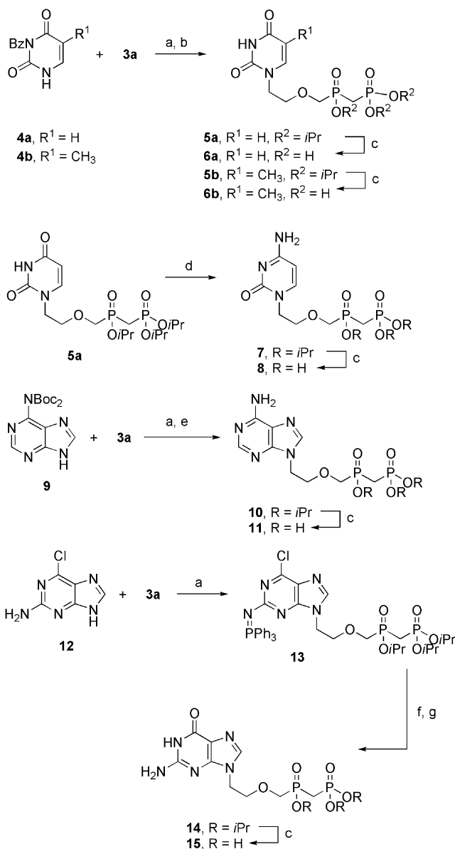
Scheme 2. Mitsunobu reaction of heterocyclic bases with alcohol 3a . Reagents and conditions: a) Ph_3P , DIAD, THF, b) MeONa, MeOH, c) BrSiMe_3 , CH_3CN , d) 1. TPSCl, CH_3CN , 2. NH_4OH , e) HCl, CH_2Cl_2 , f) H_2O , THF, g) TFAA, H_2O .
