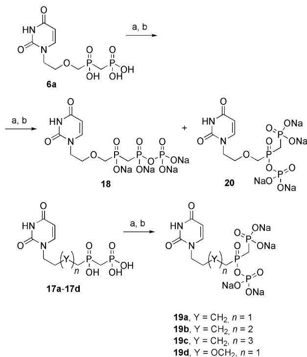
Scheme 4. Phosphorylation of compounds 6a and 17a–d . Reagents and conditions: a) 1. CDI, DMF, 2. (Bu 3 NH) 2 PO 4 , DMF, b) Dowex 50 × 8 (Na + form).
