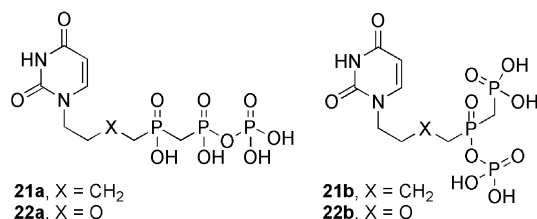
Figure 5. Molecules studied by ab initio quantum chemical calculations.
