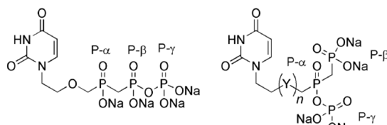
Figure 2. Labeling of phosphorus atoms for ^{31}\text{P} NMR spectroscopy.
